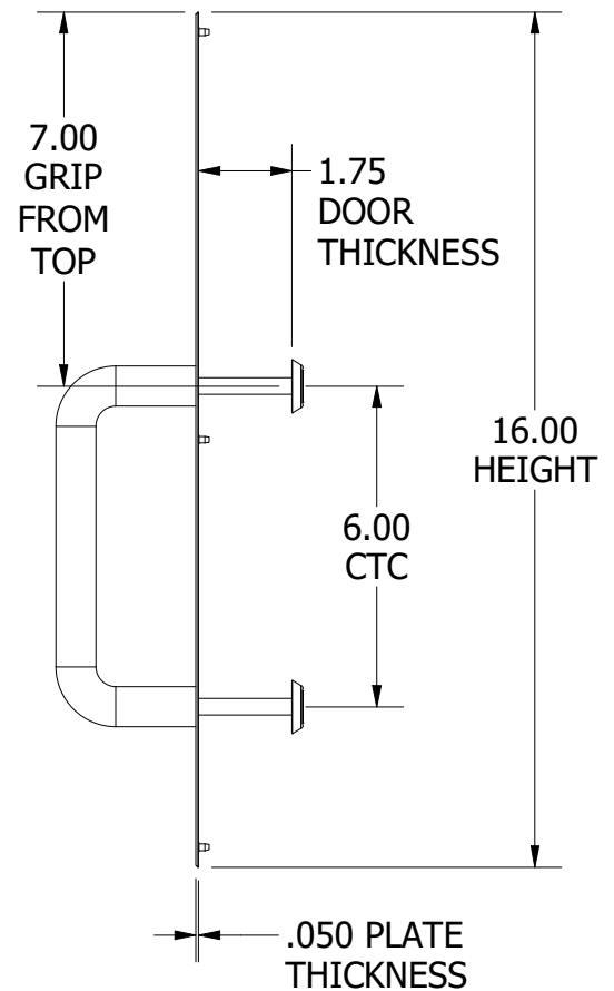
1017-2.630 ISO VIEW
